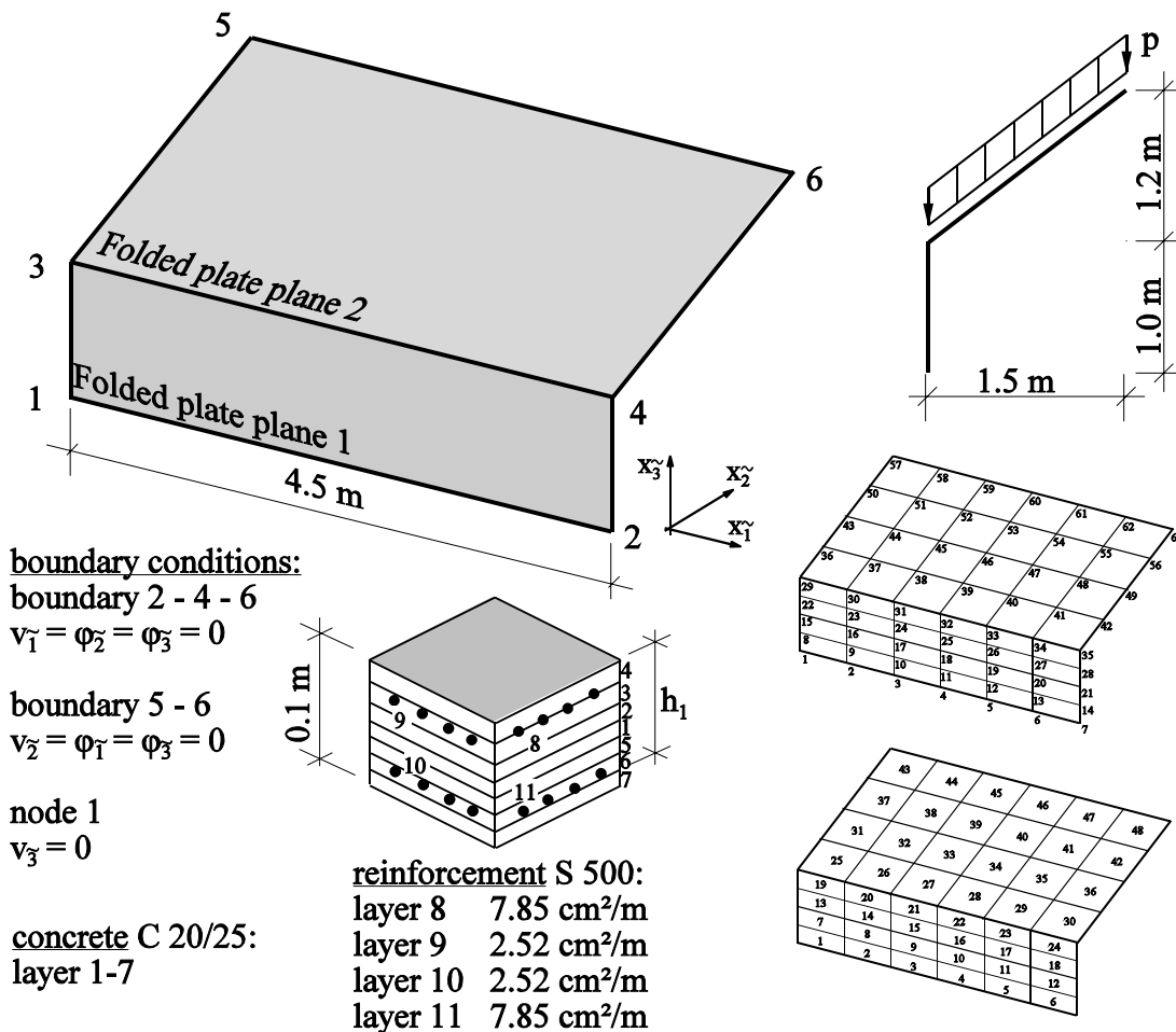
Figure 5: Geometry, finite element model
