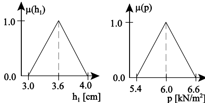
Figure 8: Membership functions of the input values
