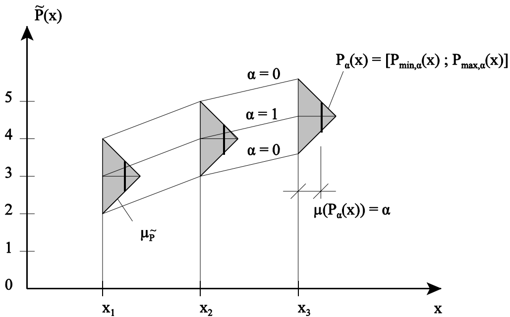
Figure 2: Approximation of the fuzzy function \tilde{P}(x) in \mathbb{R}^1 using fuzzy numbers at x_1, x_2, x_3
