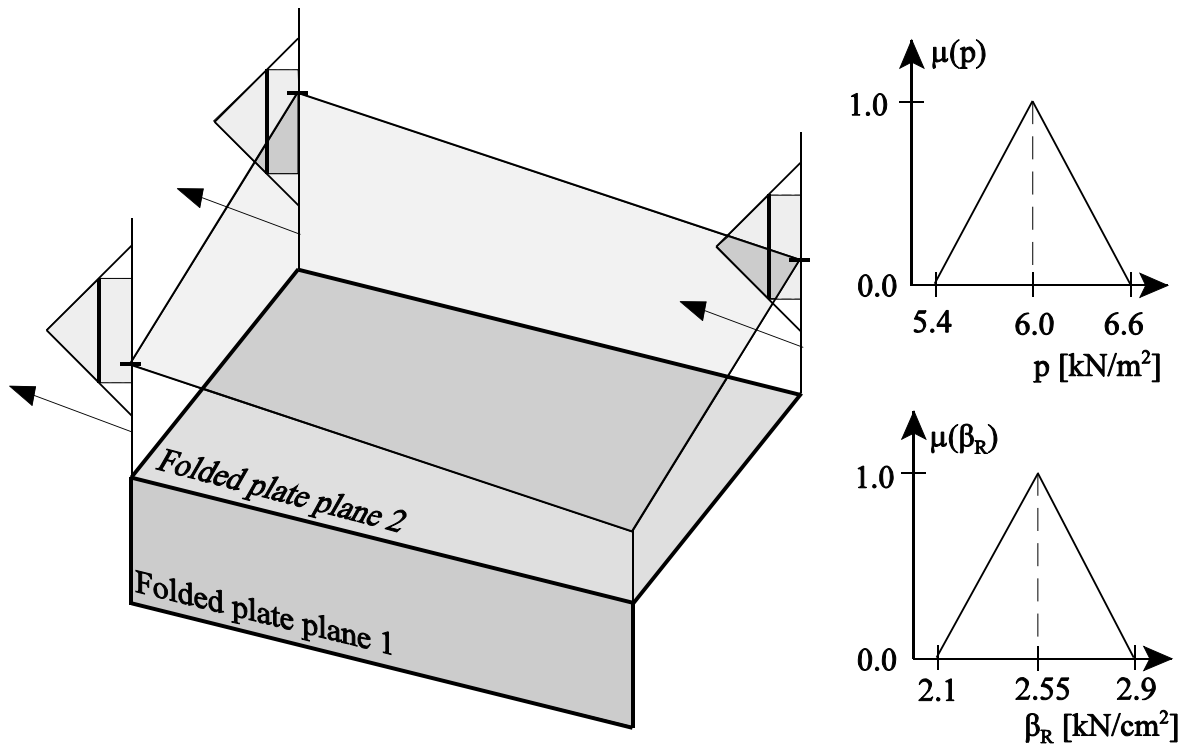
Figure 6: Fuzzy function, membership functions
